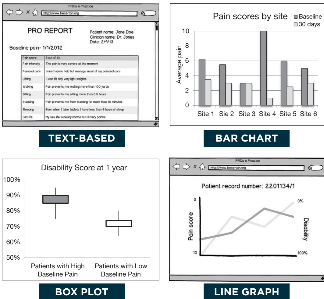
Figure 2. Wireframes for Design Cycle 1
